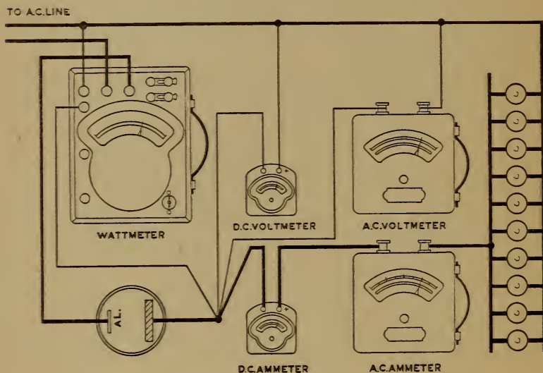
FIG. 21.—EFFICIENCY TEST OF A NODON VALVE.
